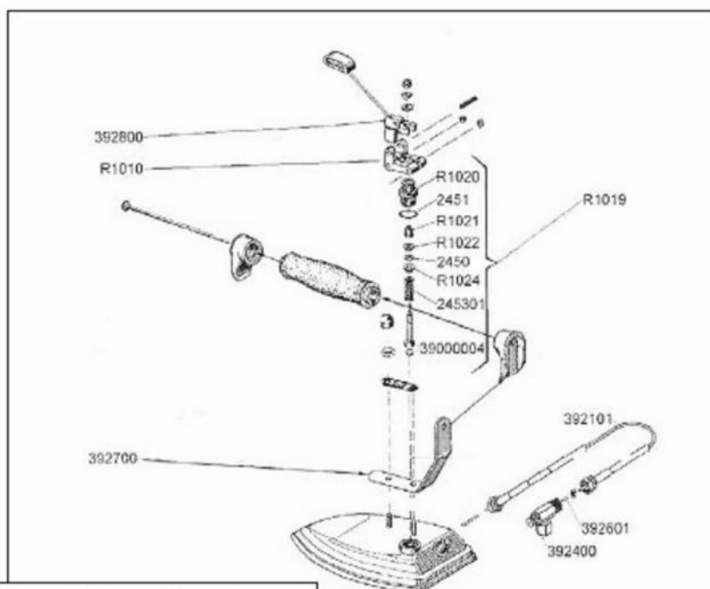
DRAWING by 2 effe Factory
