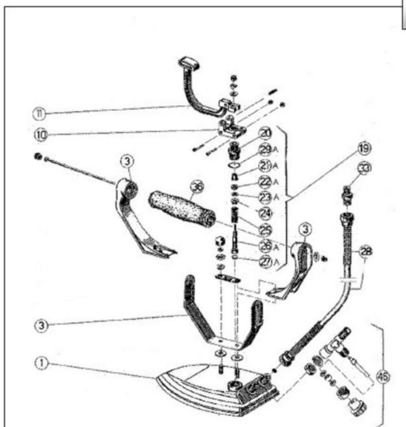
DRAWING by 2 effe Factory
